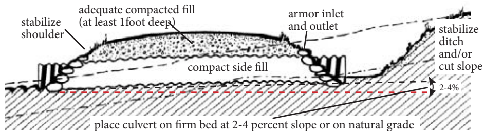
FIGURE 12A: PIPE CULVERT (CROSS-SECTION)
