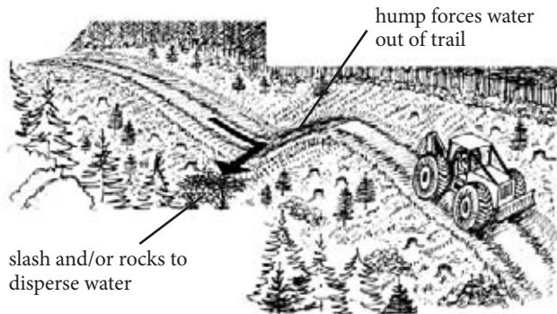
FIGURE 5: ROLLING DIP
