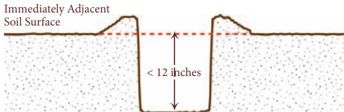
FIGURE 2: RUT CROSS-SECTION
