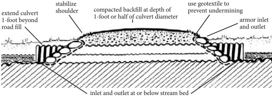
FIGURE 20: STREAM CROSSING USING PIPE CULVERT
