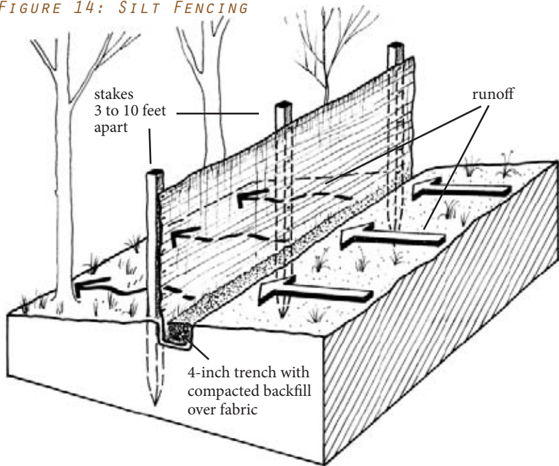
FIGURE 14: SILT FENCING
