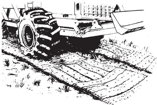
FIGURE 16: RUBBER MATS
