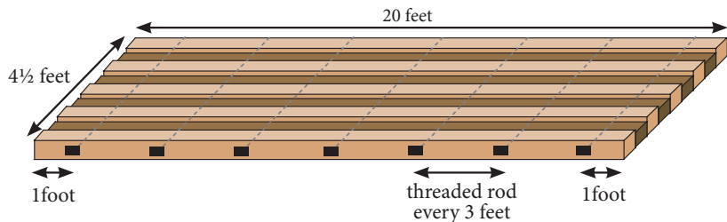
FIGURE 17: 20 FOOT SKIDDER BRIDGE PANEL CONSTRUCTION
