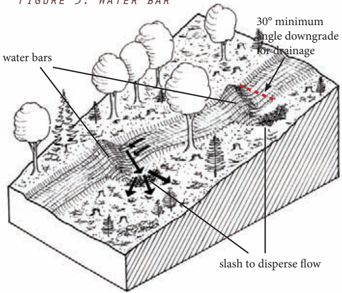
FIGURE 3: WATER BAR
