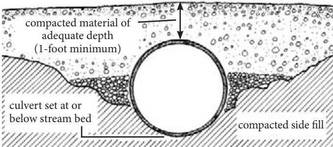
FIGURE 20: STREAM CROSSING USING PIPE CULVERT
