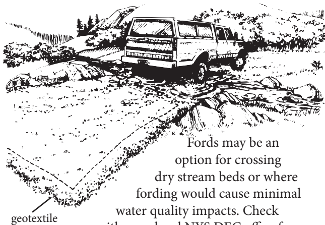
FIGURE 18: FORD CROSSING USING GEOTEXTILE
