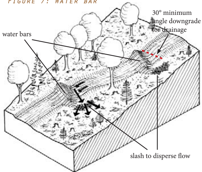
FIGURE 7: WATER BAR
