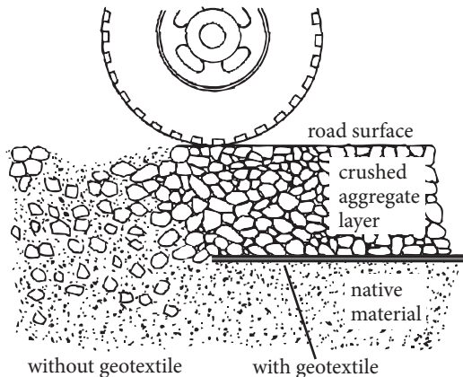
FIGURE 15: GEOTEXTILE FABRIC
