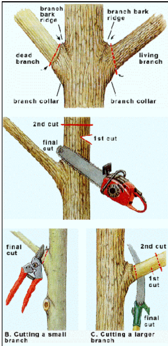
Figure 6. Pruning cuts
